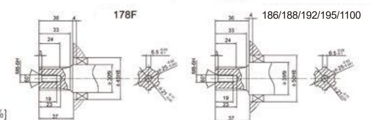
Spline shaft 花键轴
