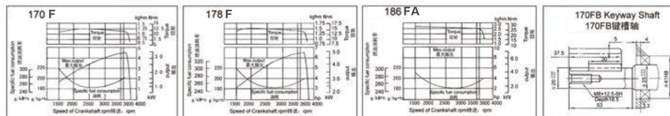
Performance Curves:性能曲线:
